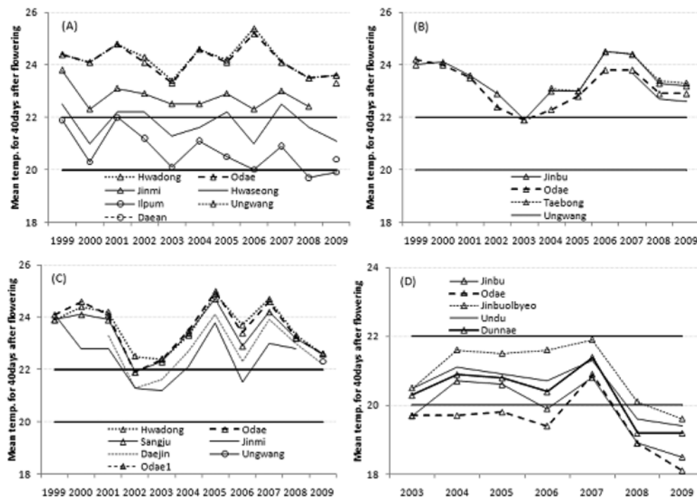
Fig. 1. Daily mean temperature for 40 days after flowering as compared with the optimum temperature range (20~22°C) in Chuncheon (A), Cheorwon (B), Gangneung (C), and Jinbu (D).
