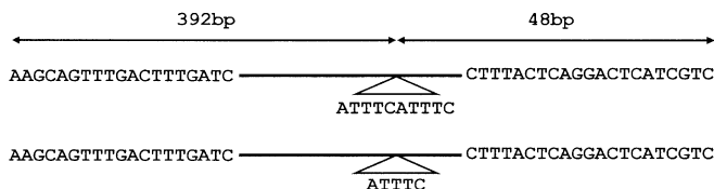
Fig. 2 Differences between large and small fragments of the Asian taxa-specific fragment shown in Fig. 1. The duplication of the penta-nucleotide, ATTTC, accounts for the size difference between them. The rest of the sequences were identical except for a few insertions or deletions
